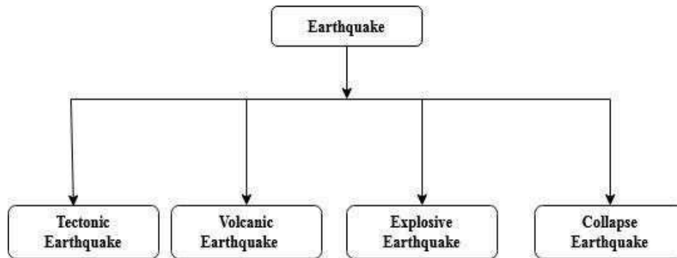
Fig. 1 – Types of Earthquakes.
