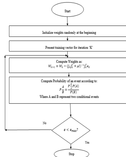
Fig.3. Flowchart for training
