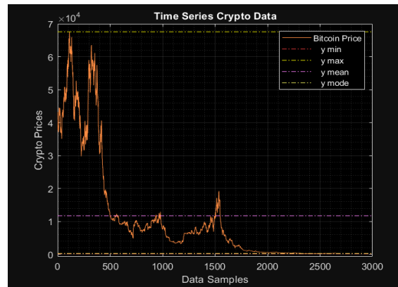
Fig.4 Original Bitcoin Price The figure above depicts variation in Bitcoin price.
