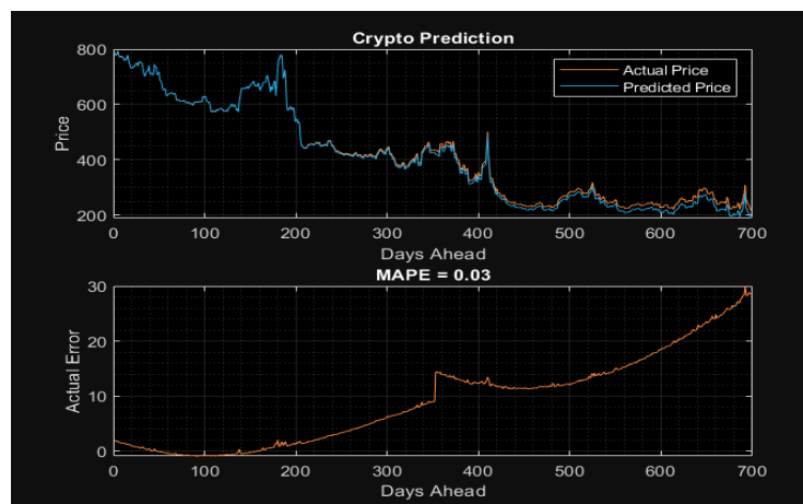
Fig.8 Predicted and Actual Crypto Behavior The figure above depicts the predicted and actual crypto behavior.
