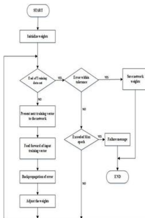
Fig.3 Flowchart of Back Propagation
