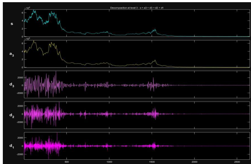
Fig. 5. Symlet Decomposition at Level 3
