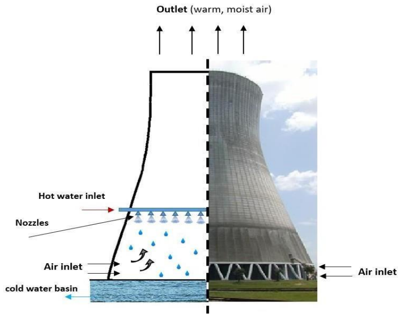
Fig. 5. Natural draft cooling tower (wet type)
