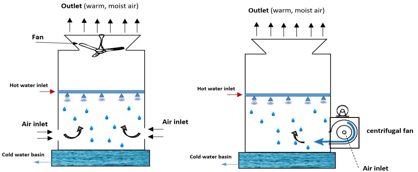
FIG. 6. Mechanical draft induced type (left) and forced type (right)
