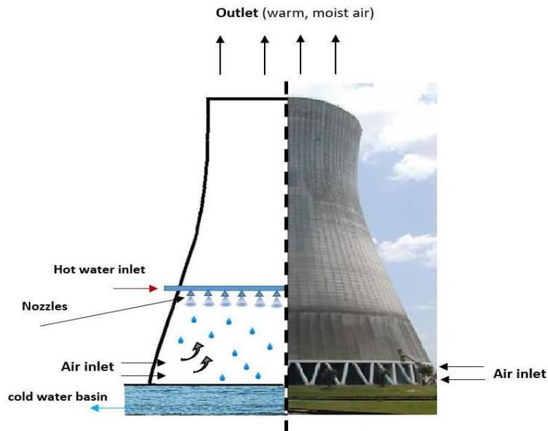
Fig. 5. Natural draft cooling tower (wet type)
