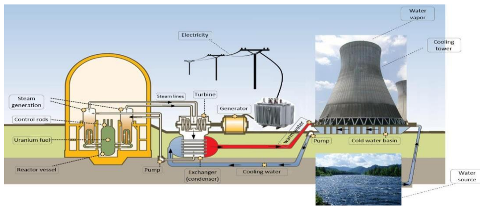
Fig. 1. A schematic view of nuclear power plant with cooling tower and main components
