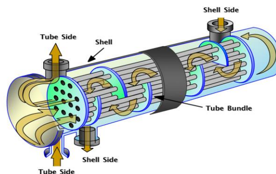
Fig.1 Shell and Tube Heat Exchanger
