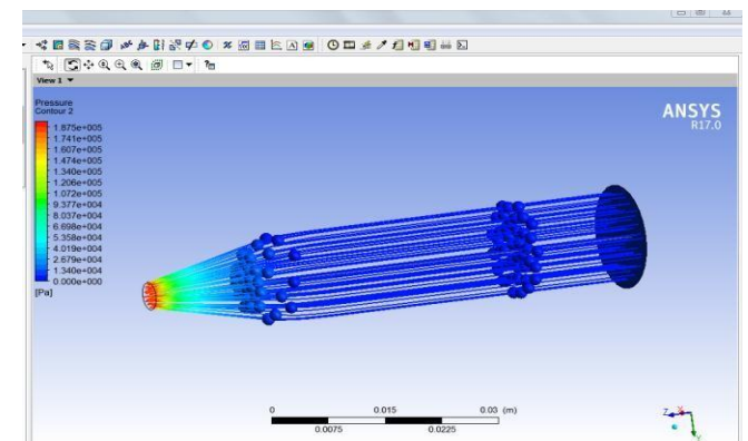
Figure: 4.4 Pressure Contour of 2mm Nozzle
