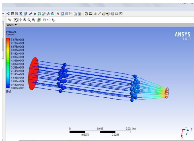
Figure: 4.9 Pressure Contour of 2.5 mm Nozzle
