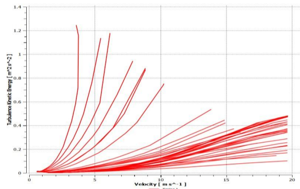
Figure: 4.6 Velocity Vs Turbulence Curve of 2 mm Nozzle
