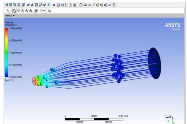
Figure: 4.2 Velocity Profile of 2mm Nozzle
