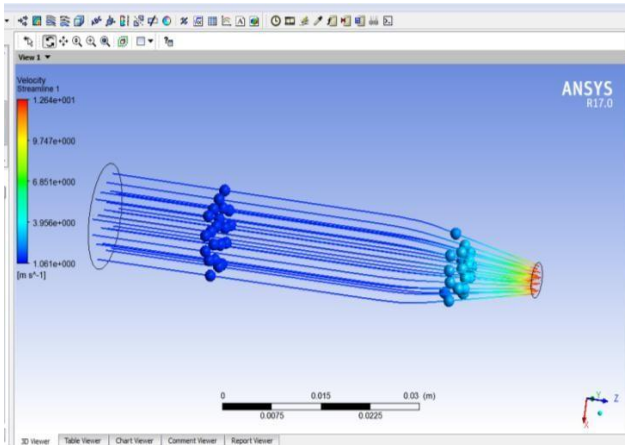
Figure: 4.7 Velocity Profile of 2.5 mm Nozzle
