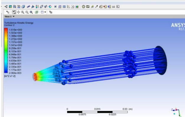
Figure: 4.5 Turbulence K.E. of 2mm Nozzle
