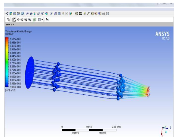
Figure: 4.10 Turbulence Kinetic Energy of 2.5 mm Nozzle
