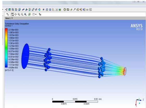
Figure: 4.8 Eddy viscosity profile of 2.5 mm Nozzle
