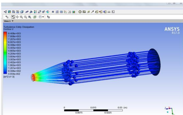
Figure: 4.3 Turbulence Eddy Dissipation of 2mm Nozzle
