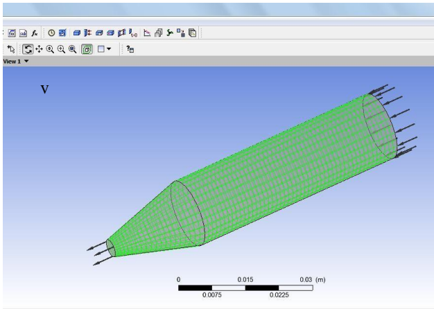
Figure: 4.1 3D model of Nozzle
