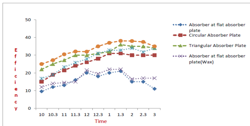
Figure No1.9. Comparison of efficiency vs time with wax, 14.04.2022
