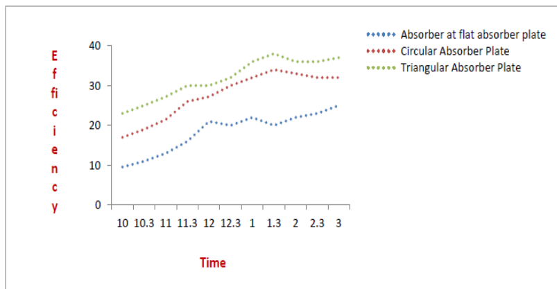
Figure No. 1.6 Comparison of efficiency vs time without wax, 14.04.2022
