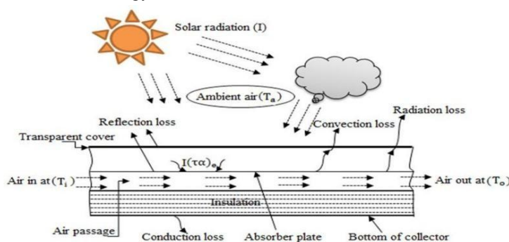
Figure No. 1.1: Conventional solar air heater.
