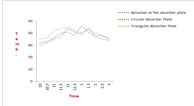
Figure No. 1.4 Comparison of efficiency vs time without wax, 13.04.2022
