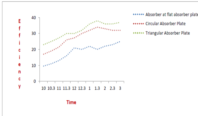
Figure No. 1.7 Comparison of efficiency vs time with wax, 13.04.2022
