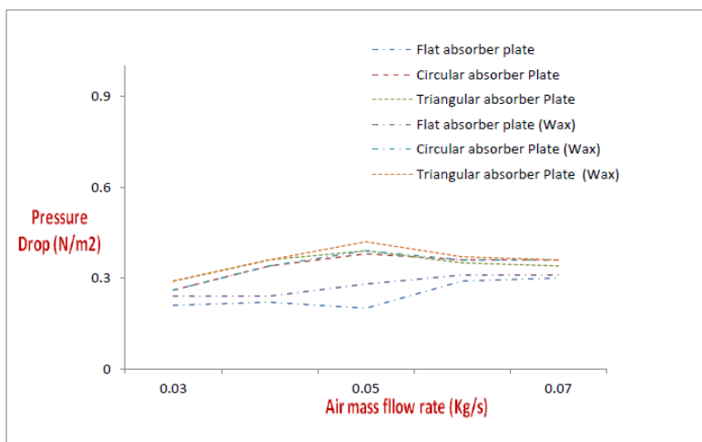
Figure No1.11 Variation of pressure drop vs air mass flow rate with wax dated 14.01.2022
