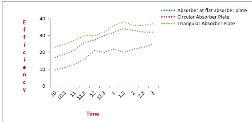
Figure No. 1.5 Comparison of efficiency vs time without wax, 13.04.2022
