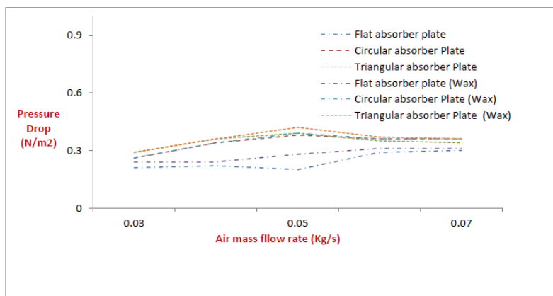
Figure No1.10 Variation of pressure drop vs air mass flow rate with wax dated 13.01.2022
