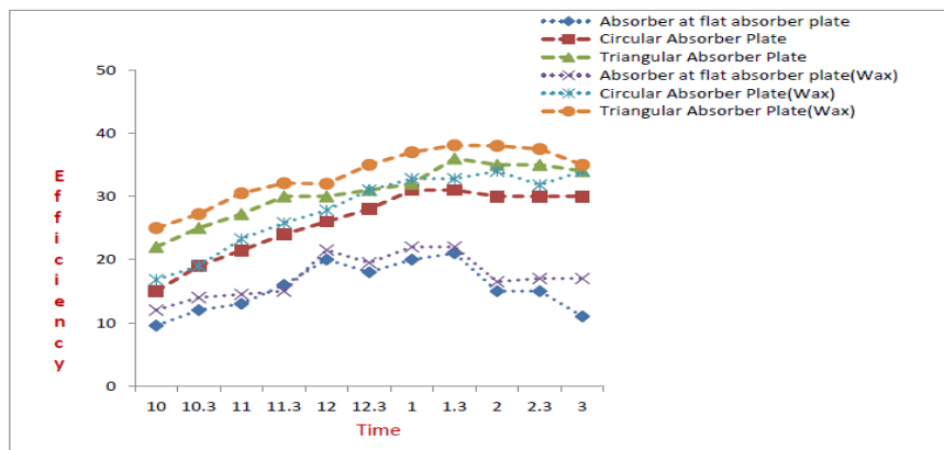
Figure No1.8. Comparison of efficiency vs time with wax, 13.04.2022
