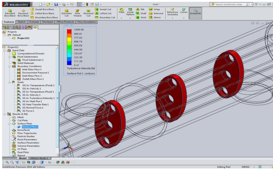
Fig.4.3 Oval Shape Baffles Turbulence Results
