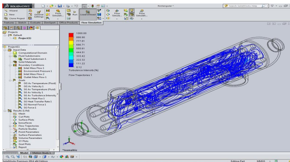
Fig.4.5 Rectangular Shape Baffles Turbulence Results
