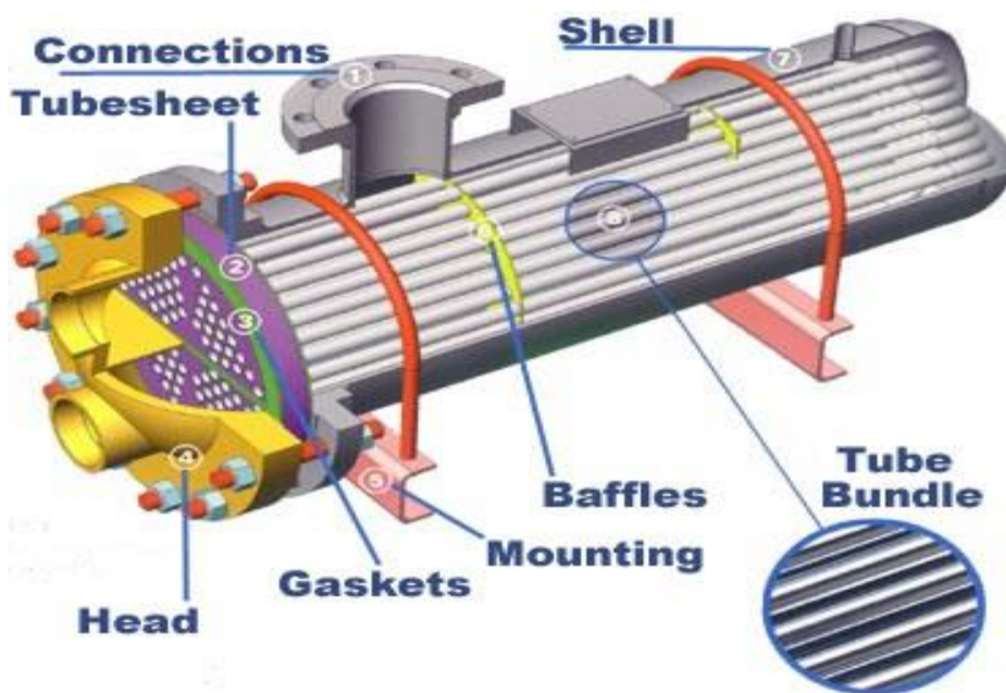
Fig.1.1 Shell and Tube Heat Exchanger
