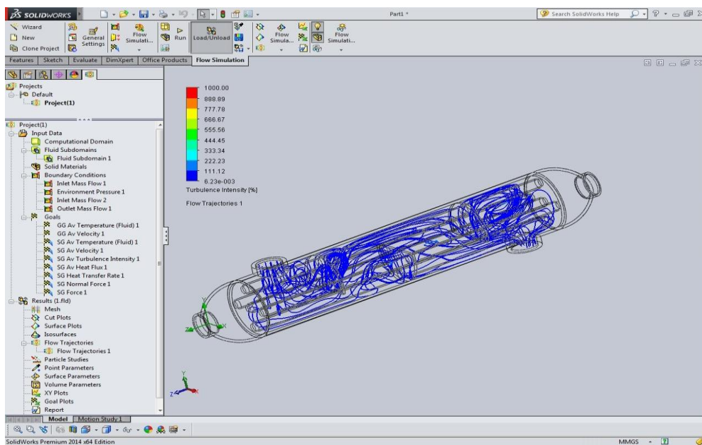
Fig.4.1 Circular Baffles Turbulence Results
