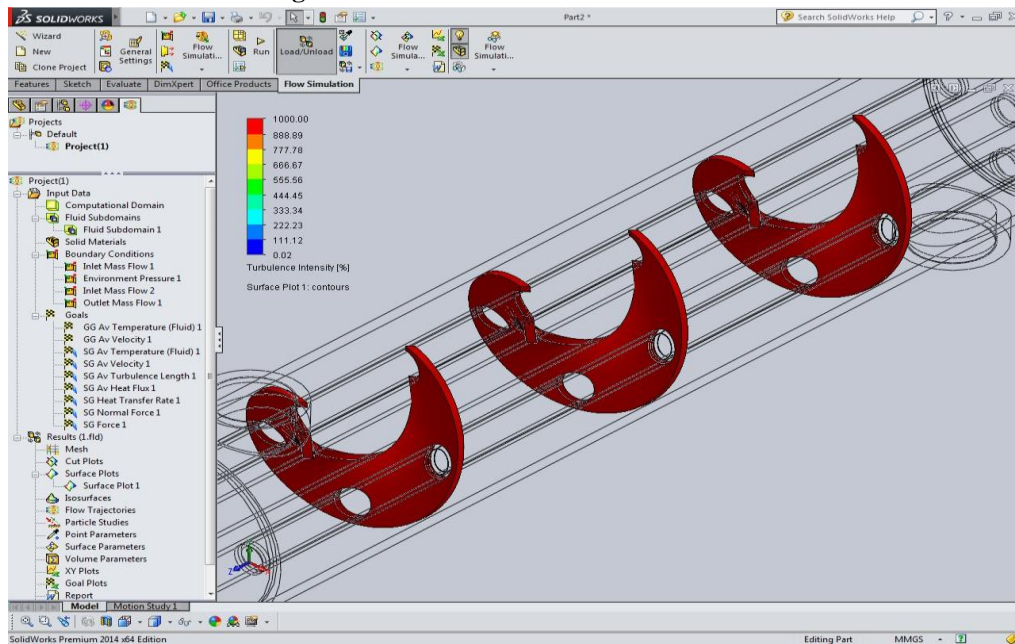
Fig. 4.2 10 degree inclined Circular Baffles Turbulence Results
