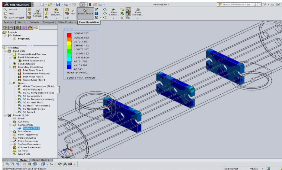
Fig.4.4 Rectangular Shape Baffles Heat flux Results
