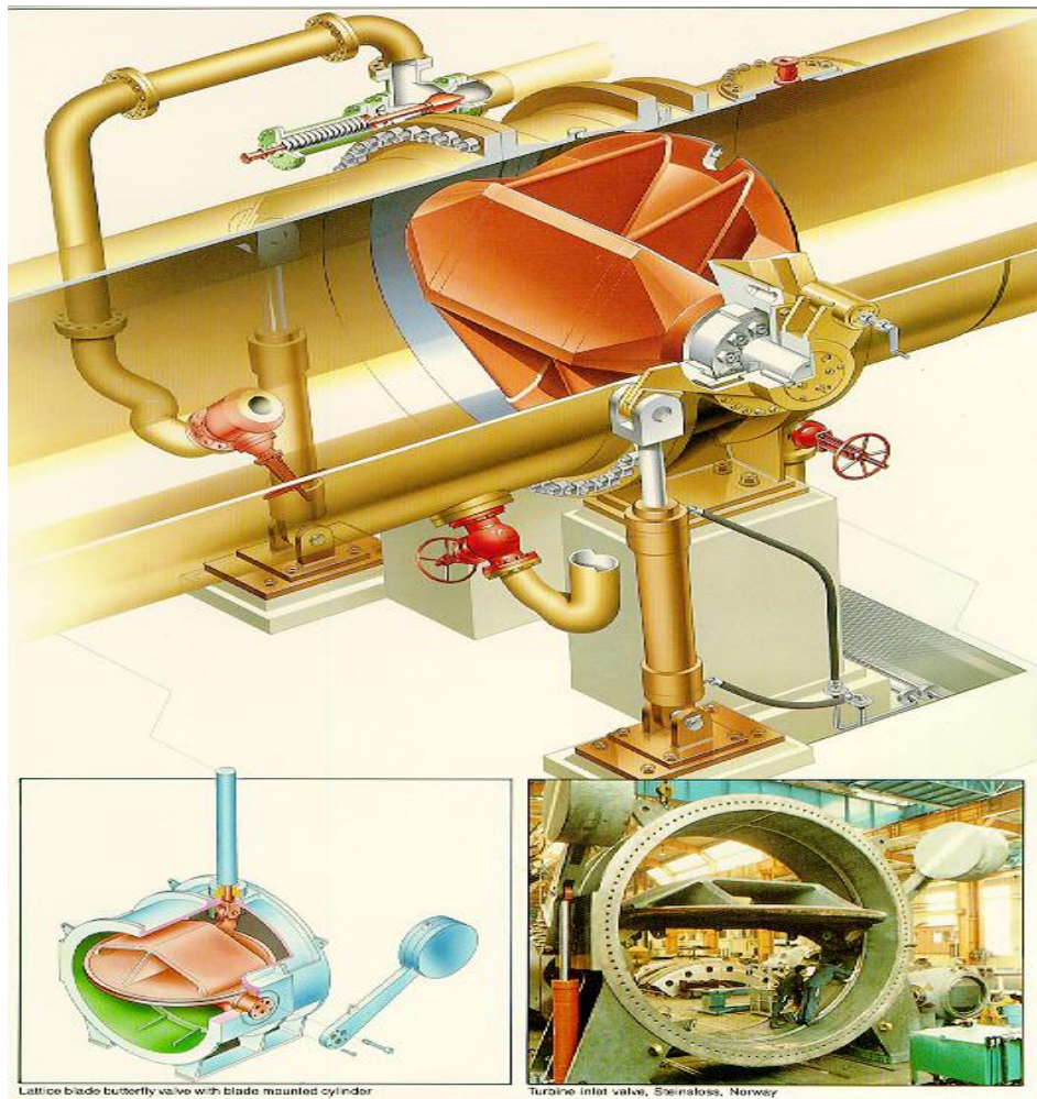
Fig.1 Turbine inlet Valve
