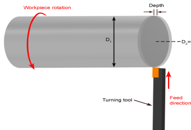
Fig.1 Turning process
