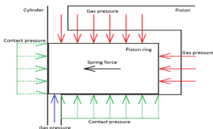
Fig.1.3 Force acting on Piston
