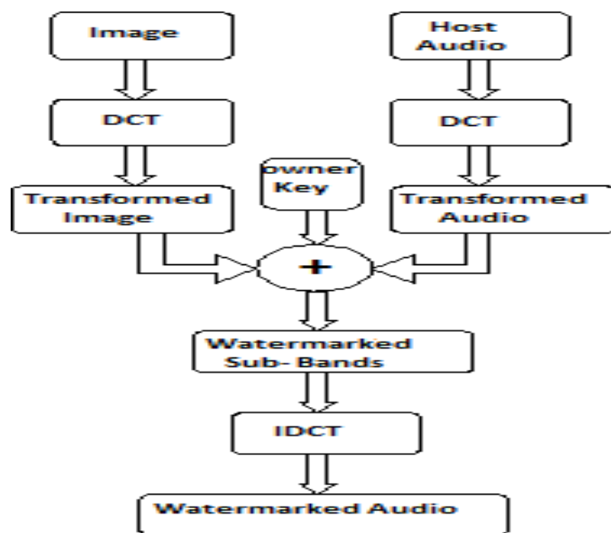
Figure 2.1 Watermark Embedding Algorithm
