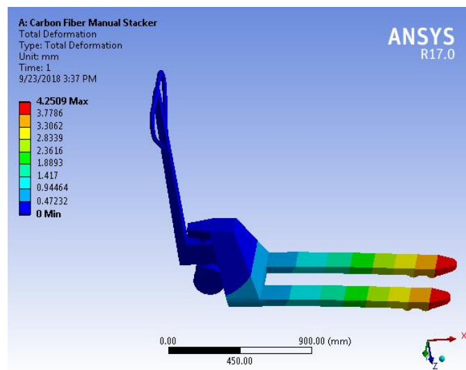
Fig.4.10 Carbon Fiber Deformation
