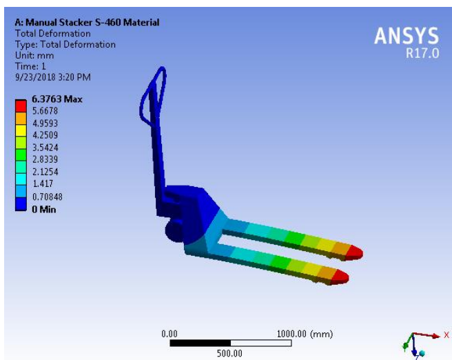
Fig.4.6 Total Deformation (Structural Steel)
