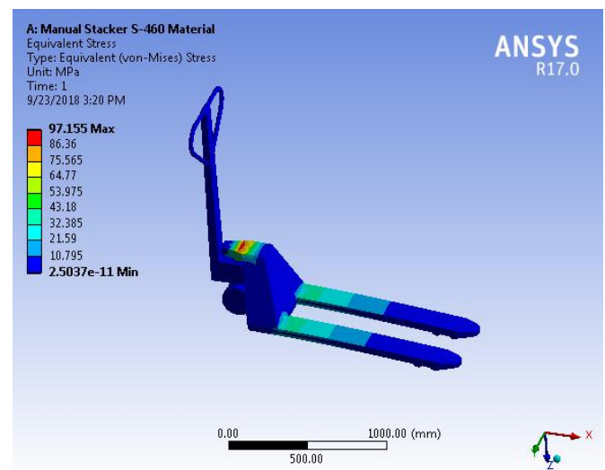
Fig.4.5 Equivalent Stress (Structural Steel)
