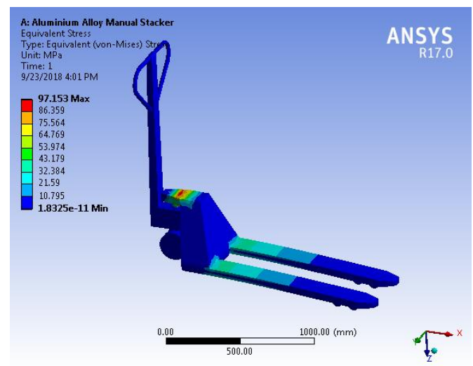
Fig.4.7 Equivalent Stress (Aluminium Alloy)
