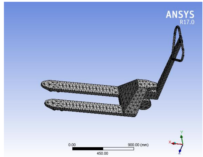
Fig.4.3 Geometry Meshing
