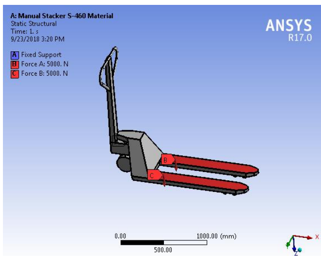
Fig.4.4 Boundary conditions (Structural Steel)
