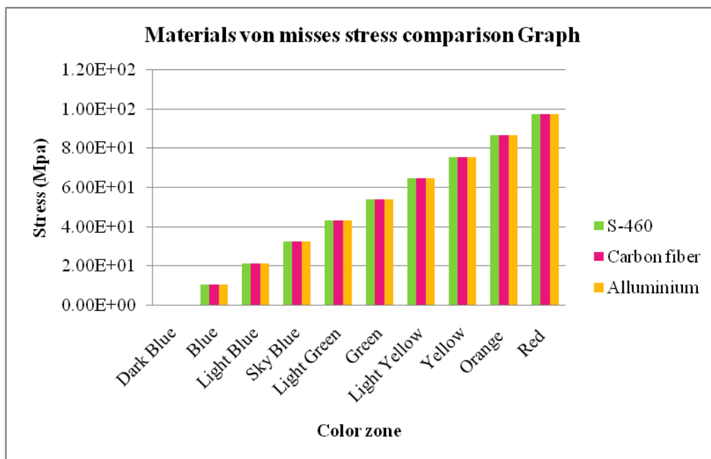
Fig.5.1 Stress comparison with different materials
