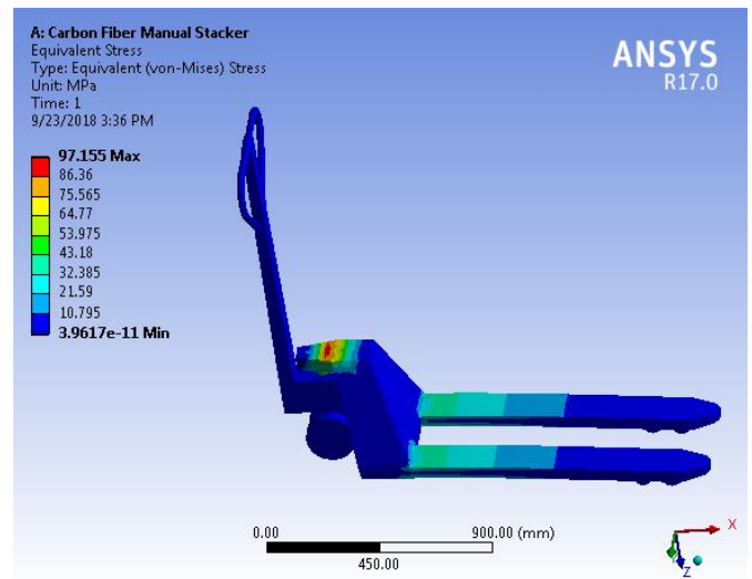
Fig.4.9 Carbon Fiber Equivalent Stress
