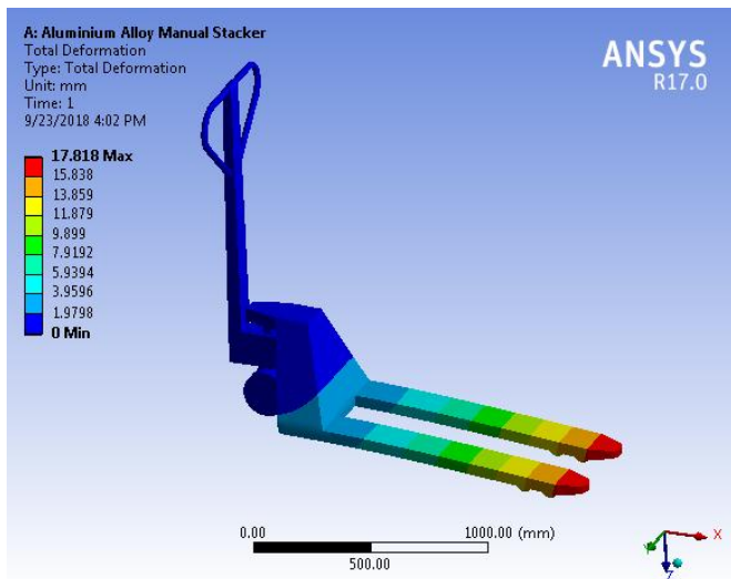
Fig.4.8 Deformations (Aluminium Alloy)
