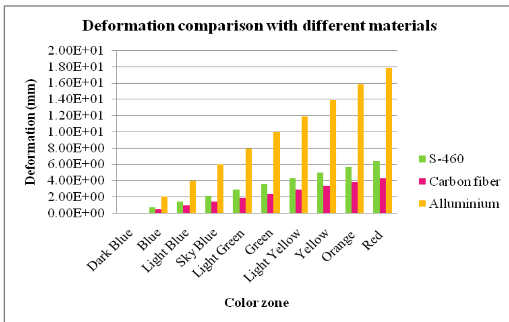
Fig.5.2 Deformations comparison with different materials
