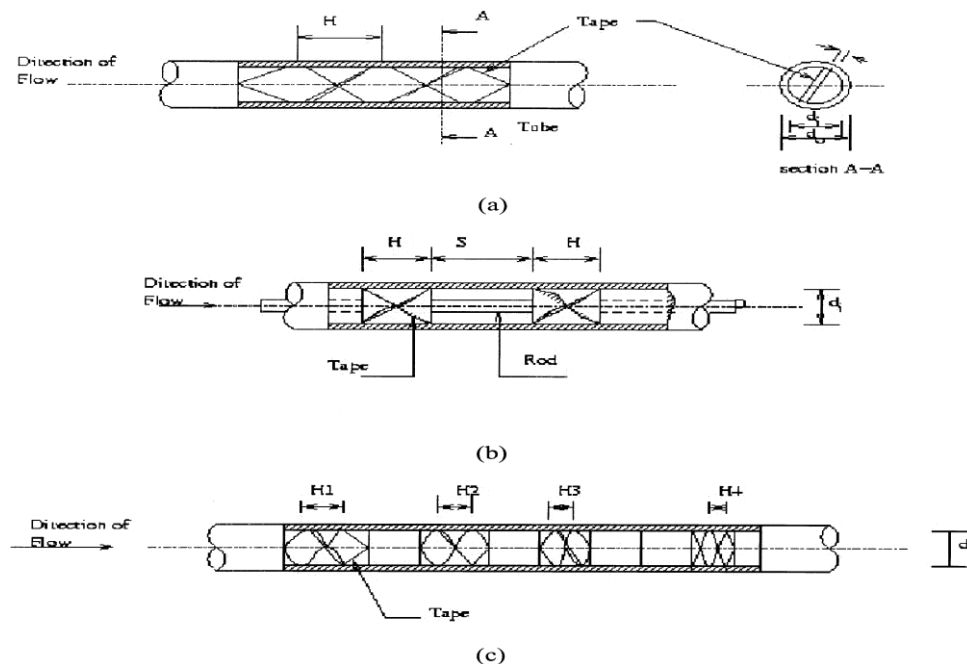
Fig:-1 (a) full-length twisted tape, (b) regularly spaced twisted tape and (c) smoothly varying (gradually decreasing) pitch full-length twisted tape.
