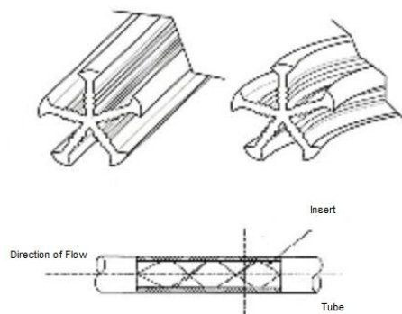
Fig:-2 Turbulent flow generator in circular tube
